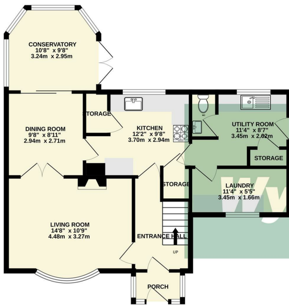
GROUND FLOOR 707 sq.ft. (65.7 sq.m.) approx.
