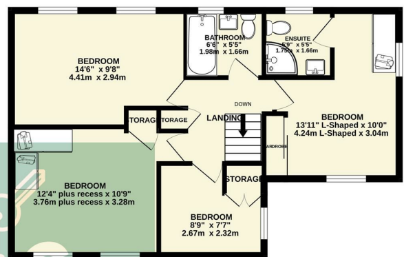
1ST FLOOR 593 sq.ft. (55.1 sq.m.) approx.
